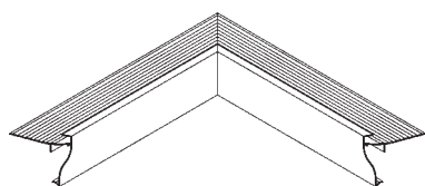
Angle rentrant Roval-Wave®
